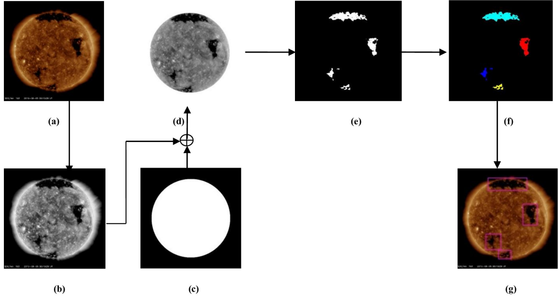
Fig. 2: Steps of ROI detection. (a) An AIA 193 Å image, (b) Converted Gray Scale image, (c) Mask Image of Image (b) for solar disk segmentation, (d) Segmented Solar Disk, (e) Supervised Thresholding, (f) Distance Transform Clustering(DTC) and Connected Component Labeling, (g) Detected ROI (CH regions).
