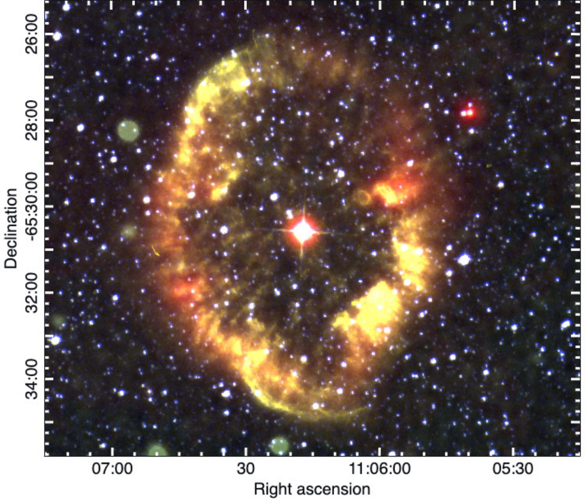
Fig. 3: Four-colour composite image of WR40 and RCW 58. Red is WISE 22 \mu\text{m} , yellow is SuperCOSMOS \text{H}\alpha , green is the EMU observation, and blue is the DSS2 red plate provided from Lasker et al. (1996) .
